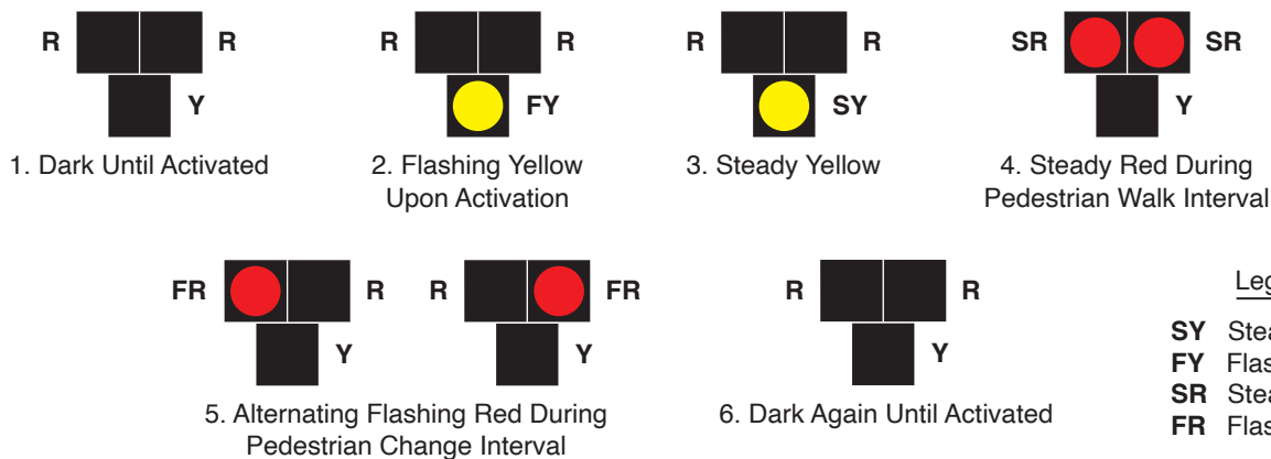
Figure 4J-3(VA). Sequence for a Pedestrian Hybrid Beacon
